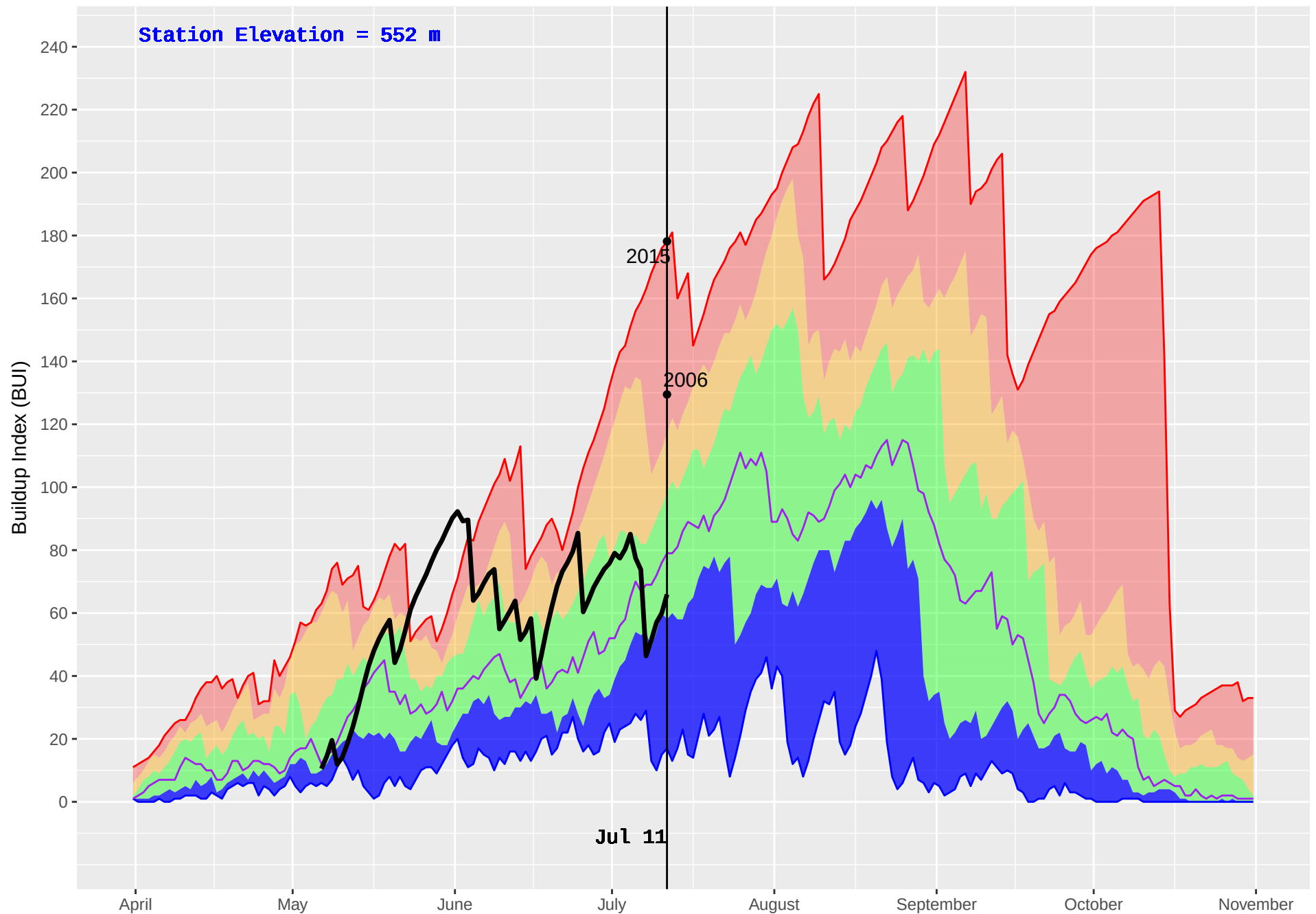
NAHATLATCH (316) : Historical (2001–2016) and Current (2018) Noon Buildup Index (BUI)
