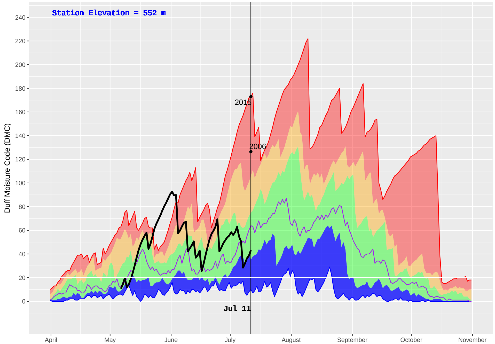
NAHATLATCH (316) : Historical (2001–2016) and Current (2018) Noon Duff Moisture Code (DMC)
